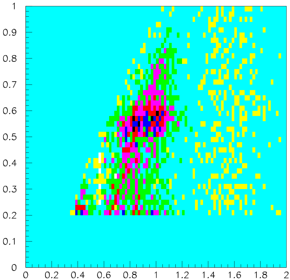
m(\gamma\gamma) vs M(3\gamma) tagged
