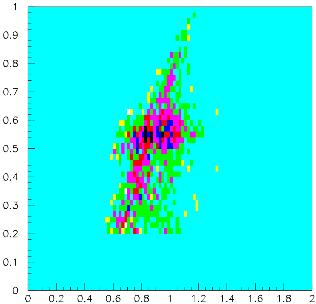
m(\gamma\gamma) vs M(3\gamma) down-tagged
