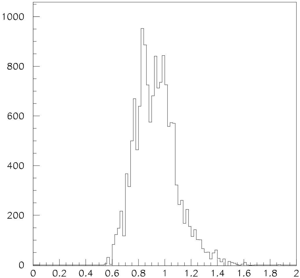
m(\gamma\gamma) vs M(3\gamma) down-tagged
