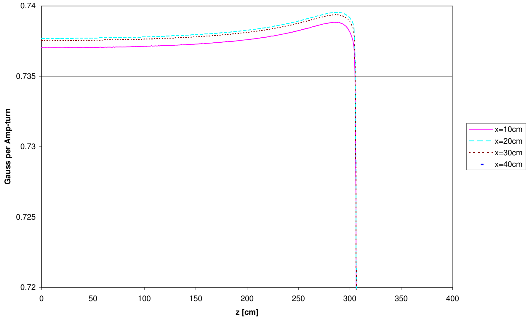
B/NI vs z at 17 kG
