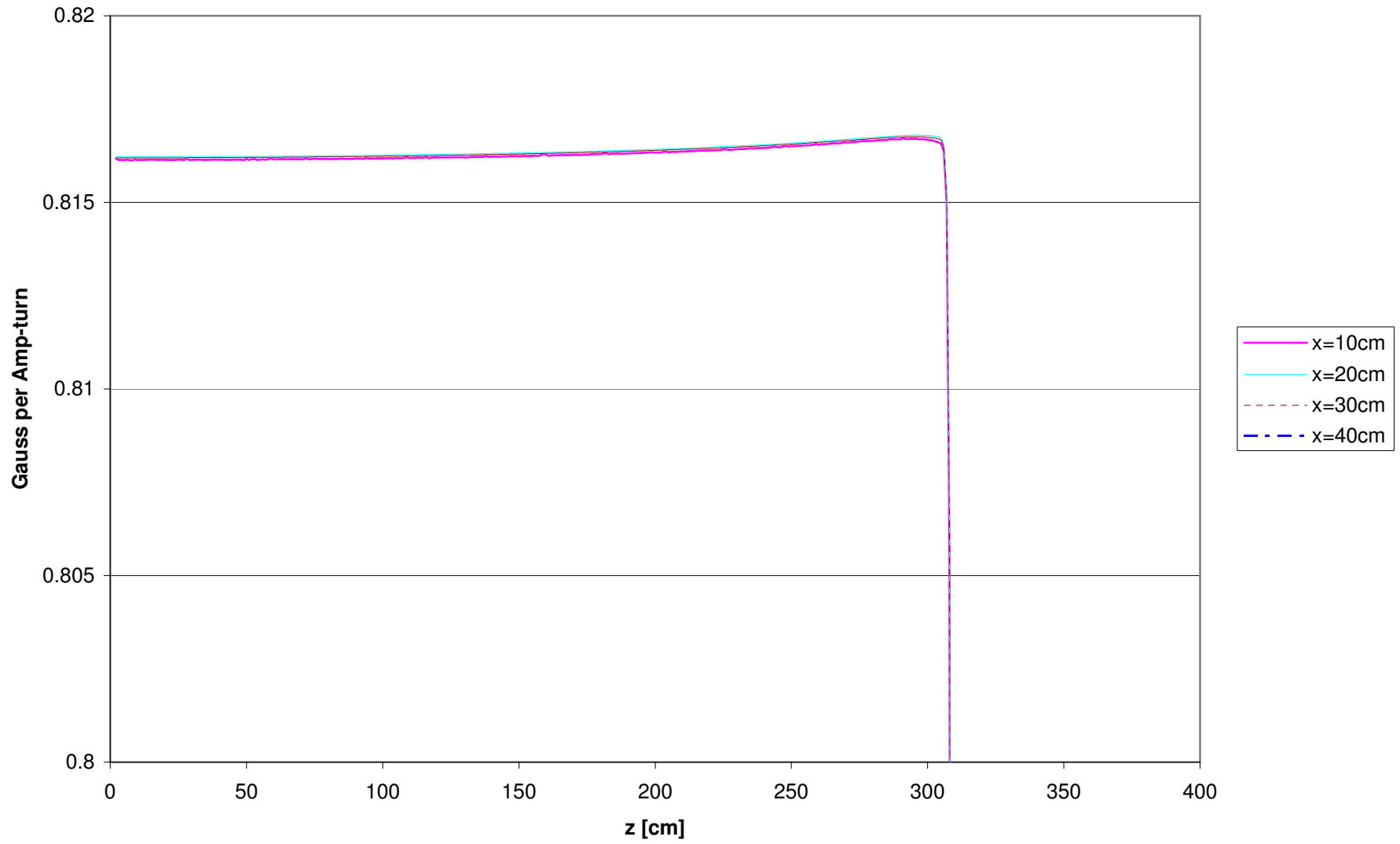
B/NI vs z at 14 kG
