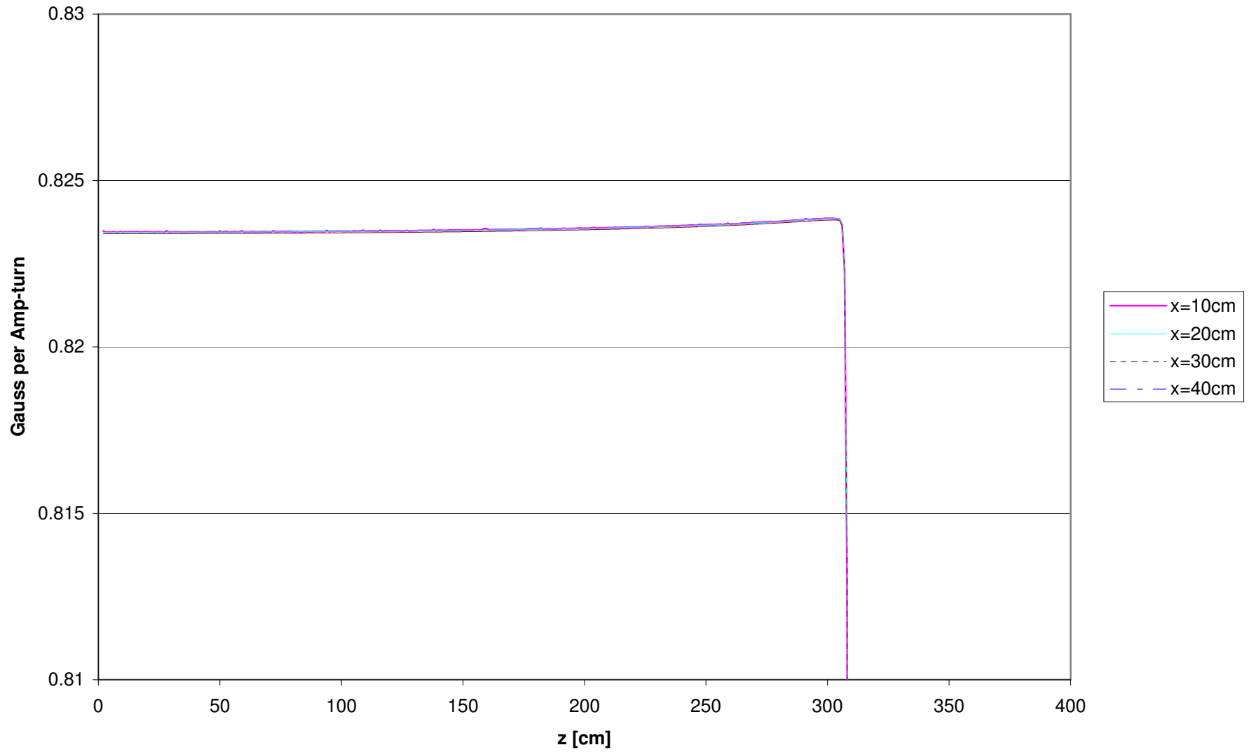
B/NI vs z at 12 kG
