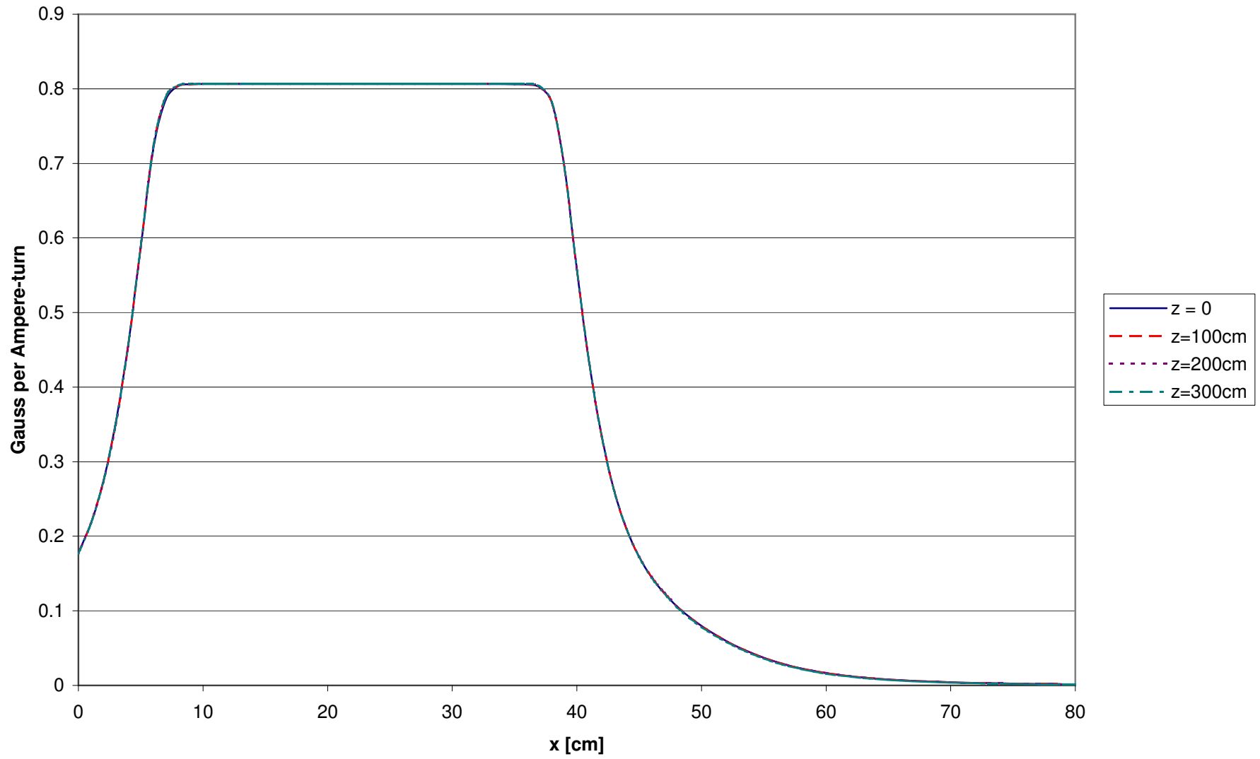
B/NI vs x at 15 kG
