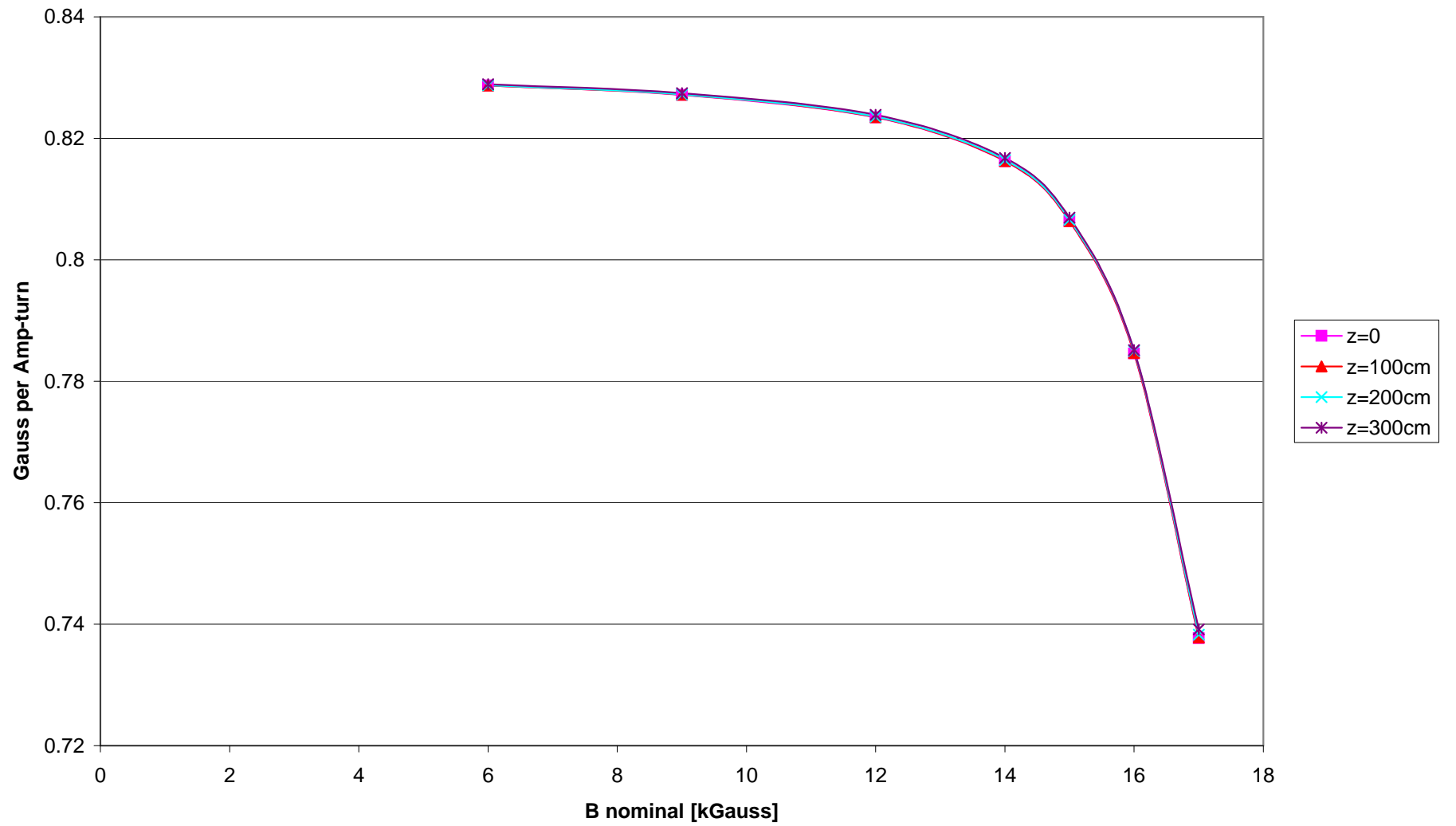
B/NI vs B_nominal at x=20cm
