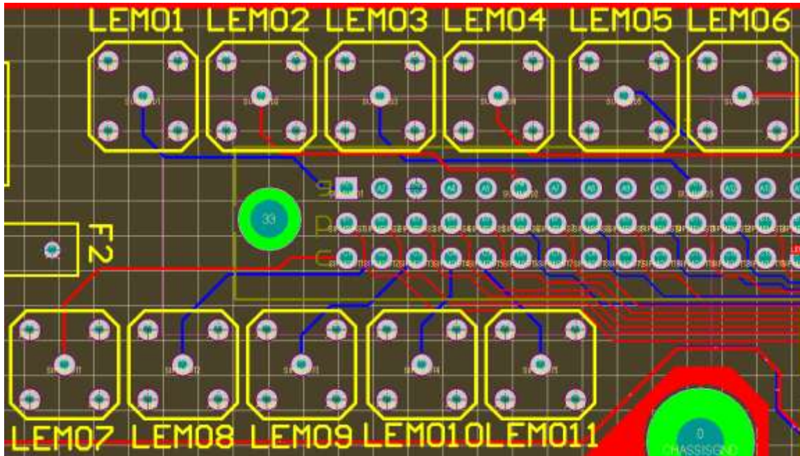
Figure 29: Close-up CAD drawing of the LEMO connectors
