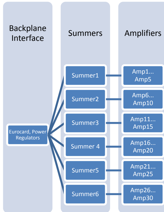
Figure 32: Hierarchy of the amplifier board circuitry
