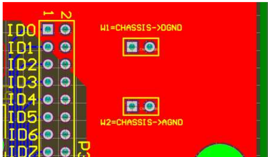
Figure 26: Close-up CAD drawing of the ground coupling jumpers on the backplane
