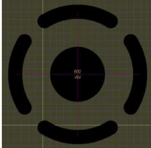
Figure 23: CAD drawing of a typical via heat relief
