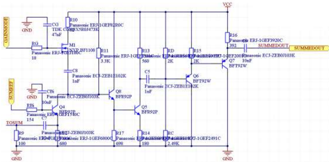
Figure 37: Schematic of the amplifier board's summing circuit
