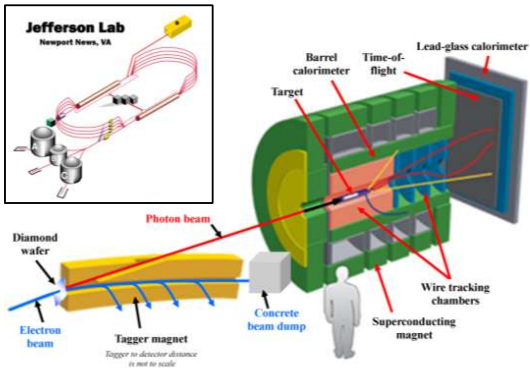
Figure 6: Cartoon overview of the GlueX experiment. Upper-left inset shows overview of JLab's accelerator, including the new Hall D where GlueX will be located
