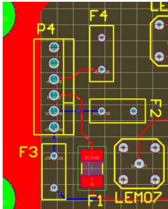
Figure 28: Close-up CAD drawing of backplane showing the power supply fuses. F1=-5V, F2=VCC, F3=+210V, F4=+5V
