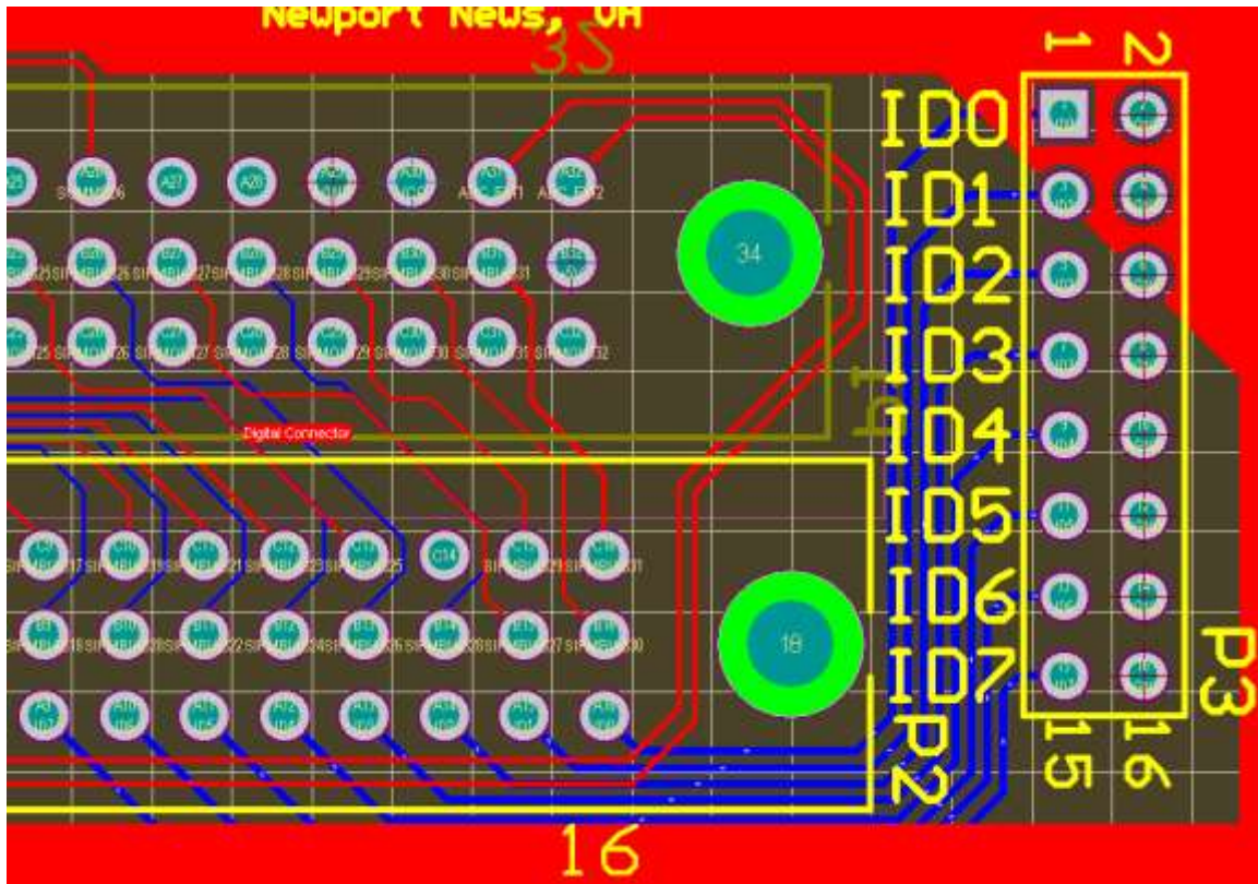
Figure 25: Close-Up CAD drawing of the Location ID bus on the backplane
