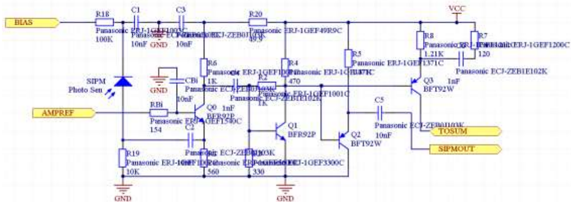
Figure 35: Schematic of the amplifier circuit
