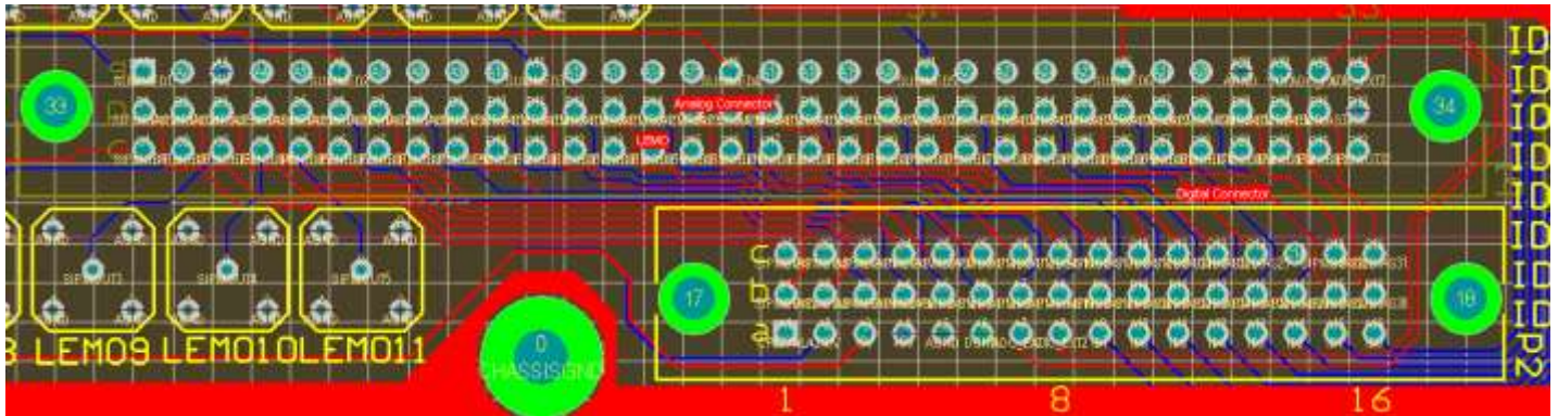
Figure 24: Close-Up CAD drawing of the Eurocard receptacle routing on the backplane
