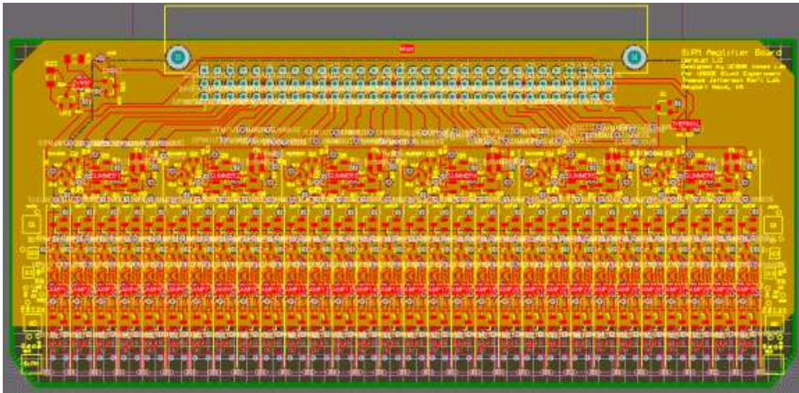
Figure 31: CAD drawing of the amplifier board
