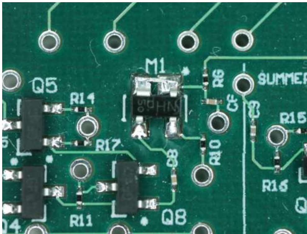
Figure 46: Photograph of the summing circuit on the amplifier board, showing the BF1108R attached to the BF1108 footprint (M1)
