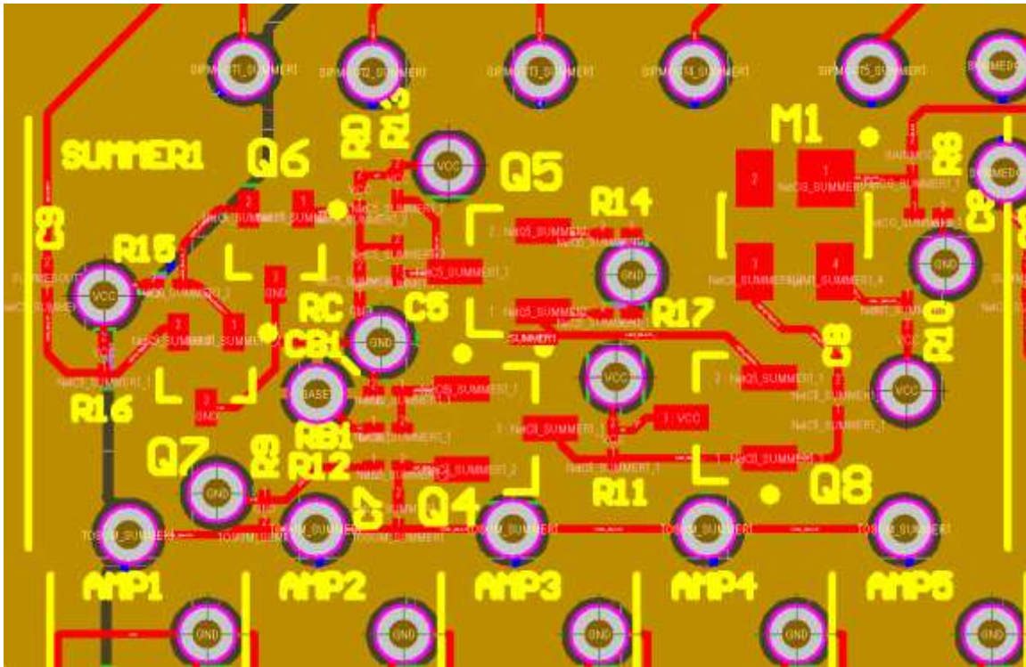
Figure 38: Close-up CAD drawing of summing circuit SUMMER1 on the amplifier board
