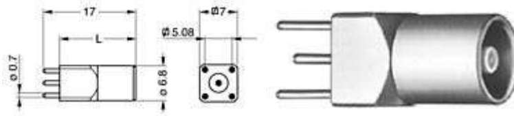
Figure 30: LEMO EPA.250.00.NTN dimensions and drawing
