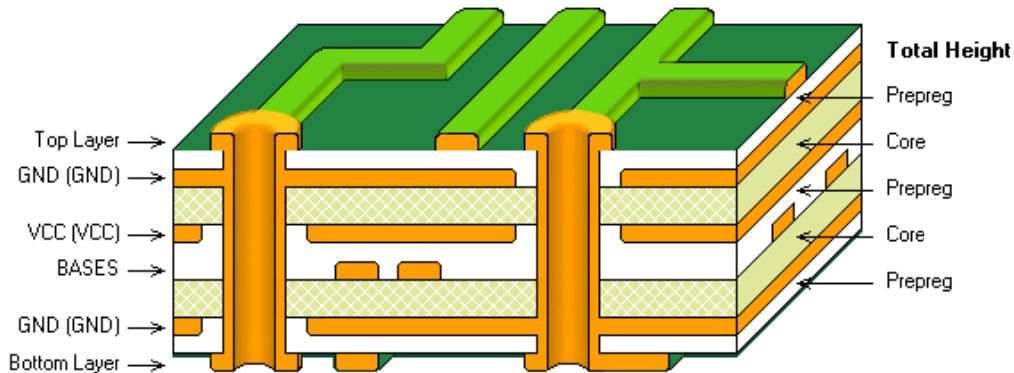
Figure 33: Amplifier board PCB layer stack-up
