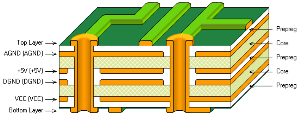
Figure 22: Drawing of backplane layer stack up
