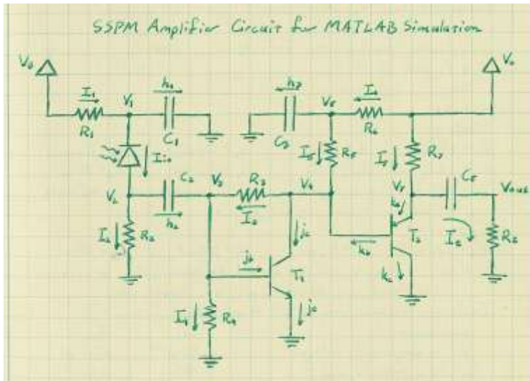
Figure 34: Schematic of AMP_0604 circuit, upon which the amplifier circuit was based
