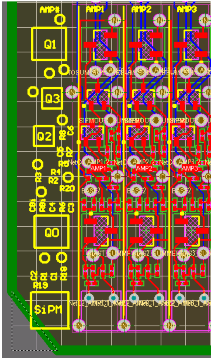
Figure 36: Close-up CAD drawing of amplifier circuitry and component key
