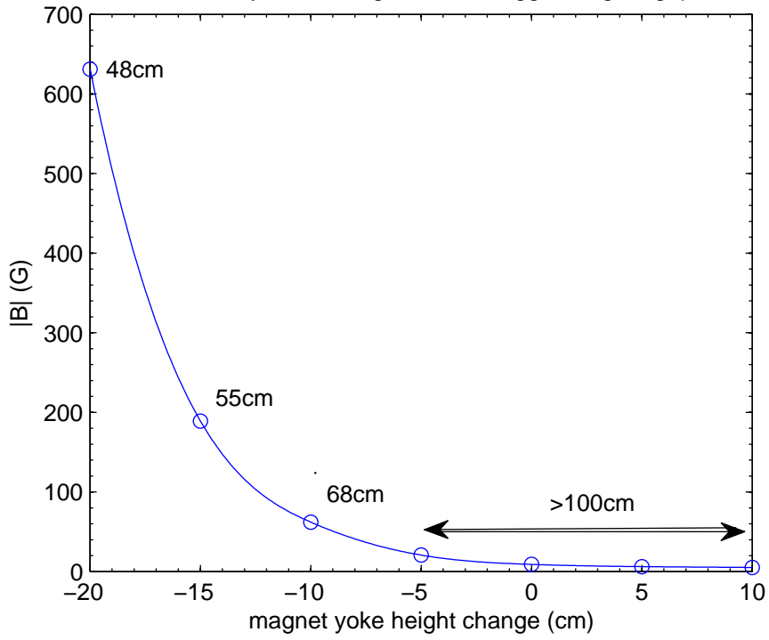
Peak stray field strength outside tagger magnet gap
