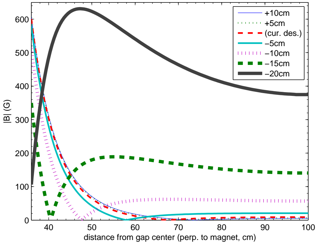
Stray fields outside tagger magnet gap
