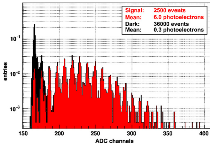
Fig. 4. The signal spectrum and the dark spectrum of a SSPM-0606EXP device during the beamtest with reflective foil. Both spectra are normalized to 1.
