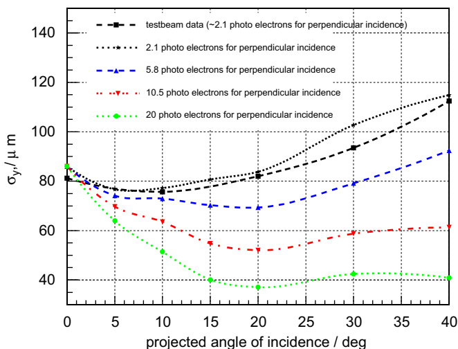
Fig. 7. Spatial resolution for a bundle of fibers of 300 μm width from testbeam data and Monte Carlo simulations. Testbeam data obtained with a fiber bundle without reflective foil and Photonique SSPM-050701GR SiPM readout are plotted using square markers. Results from Monte Carlo simulations are added to study the behavior for improved photo electron yields. A yield of 5.8 photo electrons was reached in the testbeam with SSPM-0606EXP SiPMs and reflective foil, but only data at 0° were taken in this configuration.
