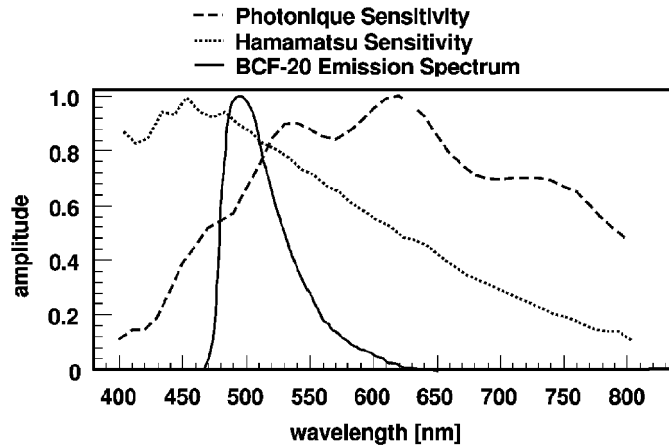
Fig. 1. Emission spectrum of a BCF-20 fiber [6] in comparison to the wavelength dependent response functions of a Hamamatsu SiPM (model MPPC S10361-025U) and a Photonique SiPM (model SSPM-0606EXP) [8].
