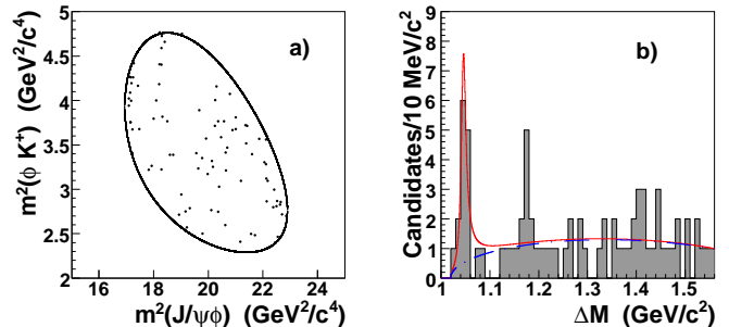
FIG. 2: (a) The Dalitz plot of m^2(\phi K^+) versus m^2(J/\psi\phi) in the B^+ mass window. The boundary shows the kinematic allowed region. (b) The mass difference, \Delta M , between \mu^+\mu^-K^+K^- and \mu^+\mu^- , in the B^+ mass window. The dash-dotted curve is the background contribution and the red solid curve is the total unbinned fit.
