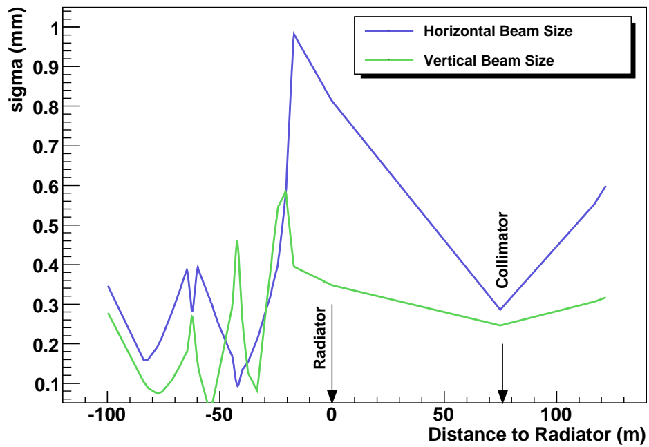
Figure 4.2: Horizontal and vertical r.m.s. envelopes for the electron beam in the region of the photon source. The origin of the z coordinate has been placed at the radiator. In the region between the radiator and the collimator the envelope refers to the projected image of the electron beam, and does not describe the size of a physical beam that exists in that region.
