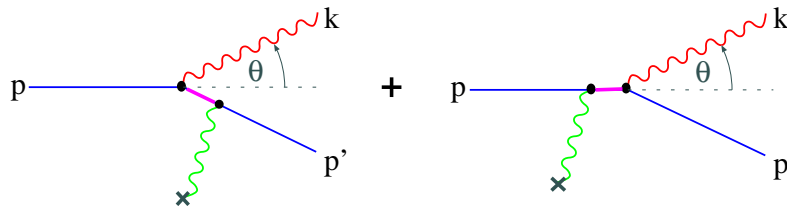
Figure 4.1: Generic diagrams for hard photon production from a high energy electron beam. The symbol \times represents either a static charge distribution, in the case of virtual photons in the initial state (i.e. bremsstrahlung), or an optical cavity, in the case of real photons in the initial state (i.e. Compton scattering).
