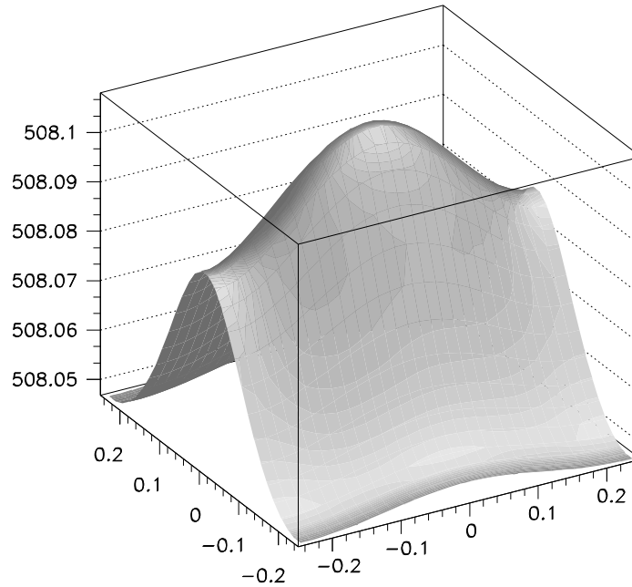
Figure 4.15: Calculated temperature profile of diamond crystal with a 12 GeV beam at 3 \mu A . The crystal dimensions are 5 \text{ mm} \times 5 \text{ mm} \times 15 \mu\text{m} . The ambient room temperature was taken to be 27^\circ \text{C} (300 K). The x-y asymmetry is caused by the elliptical shape of the electron beam spot on the radiator.
