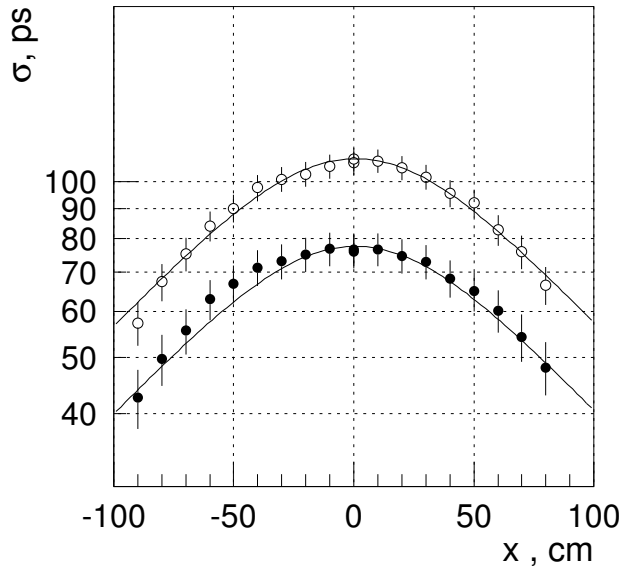
Figure 6.66: The time resolution for one (o) and two (•) 1.25 \times 6.0 \text{ cm}^2 bars viewed by XP2020 PMT's.
