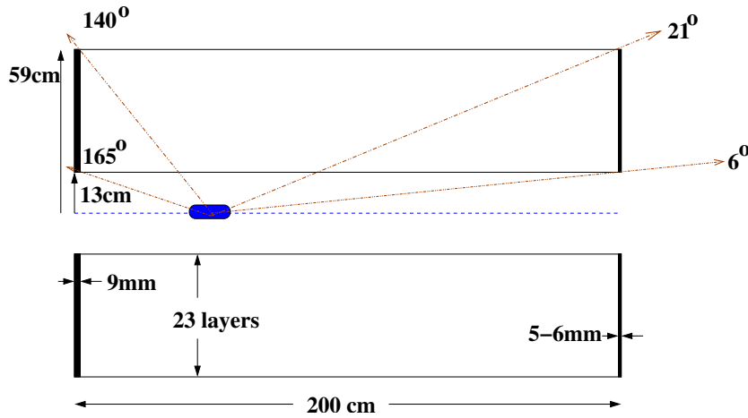
Figure 6.33: A side view sketch of the CDC.
