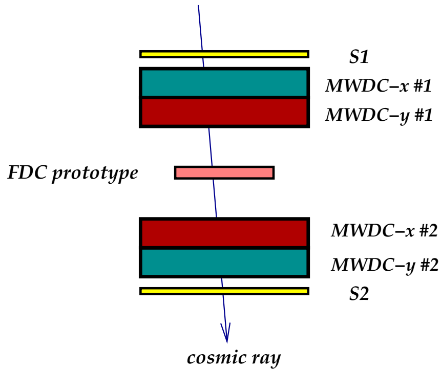
Figure 6.52: Schematic drawing of the cosmic-ray telescope used for FDC prototype resolution studies.
