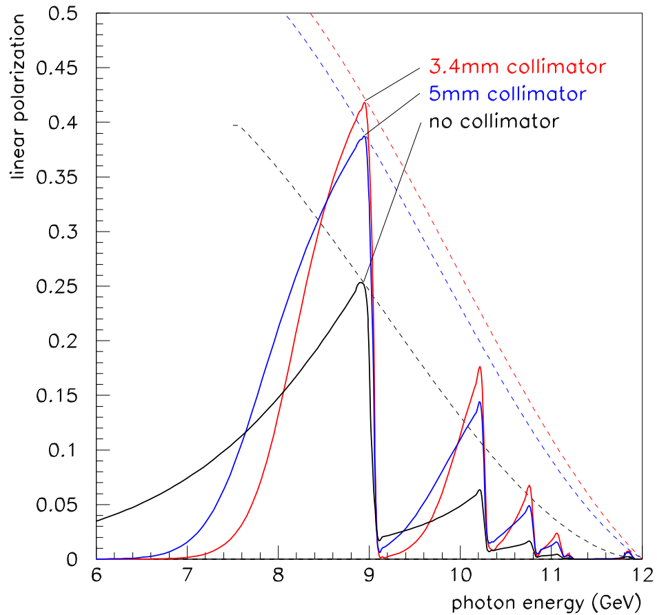
Figure 4.8: Linear polarization of the coherent bremsstrahlung beam for a fixed electron beam energy of 12 GeV calculated under the same conditions as in Fig. 4.6. The dashed lines indicate the trajectory of the peak polarization as the peak energy is swept across the focal plane by rotating the crystal.
