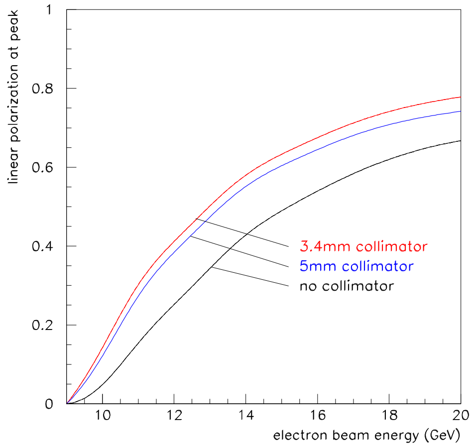
Figure 4.7: Linear polarization in the coherent bremsstrahlung peak as a function of electron beam energy keeping the energy of the coherent peak fixed at 9\text{ GeV} . The calculation is performed under the same conditions as in Fig. 4.6.
