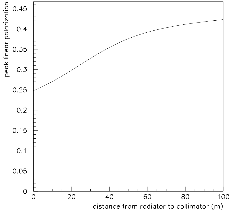
Figure 4.9: Maximum polarization vs radiator-collimator distance for a coherent peak at 9 GeV. The collimator diameter is held fixed in this calculation to keep a constant ratio between the sizes of the virtual electron spot and the collimator.
