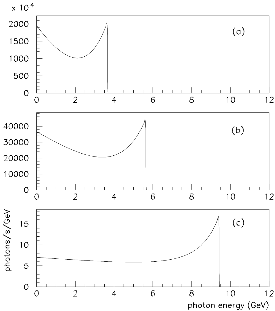
Figure 4.2: Photon energy spectrum from the Compton back-scatter source described in the text and a 12 GeV electron beam at 1\mu\text{A} . (a) cavity of gain 10000 driven by a 10kW Argon-ion laser (514 nm) pulsed at 100 MHz. (b) cavity of gain 250 driven by 3kW frequency-doubler (257 nm) pulsed at 100 MHz. (c) cavity of gain 1 driven by a hypothetical FEL source operating at 20 eV with the same time structure as CEBAF beam, peak power 1kW.
